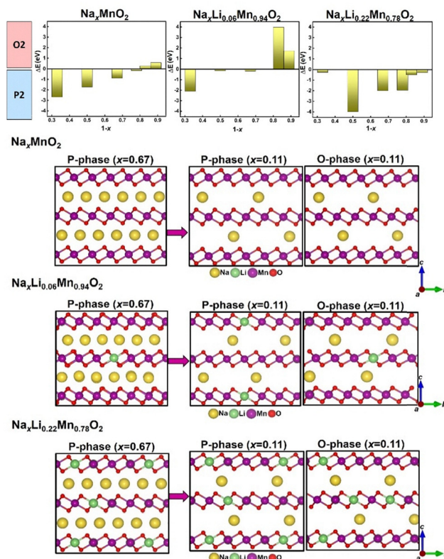
Fig. 1 (top) Computed electrostatic energy difference between the P2 and O2 phase \Delta E \text{ (eV)} = E_{\text{tot}}^{\text{P2}} - E_{\text{tot}}^{\text{O2}} versus Na-concentration using the Ewald summation (with point charges). (bottom) Side views of atomistic structures.
