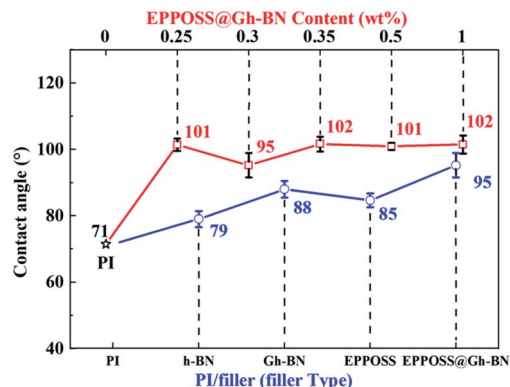
Fig. 8 Contact angles of the PI nanocomposite films with different fillers and PI/EPPOSS@Gh-BN with different filler contents.
