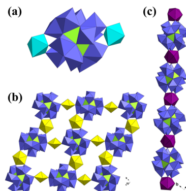
Fig. 7 Views of the Silvertone-type \{\text{UMo}_{12}\} -based structures. (a) [(\text{VO})_2(\text{H}_2\text{O})_4(\text{UMo}_{12}\text{O}_{42})]^{4-} ; (b) [(\text{UO}_2)_2(\text{H}_2\text{O})_3\{\text{UMo}_{12}\text{O}_{42}\}]^{4-} ; (c) [\text{Th}(\text{H}_2\text{O})_3(\text{UMo}_{12}\text{O}_{42})]^{4-} . Color codes: Mo, blue; \text{U}^{\text{IV}} , light green; \text{U}^{\text{VI}} , yellow; \text{Th}^{\text{IV}} , violet; V: turquoise.
