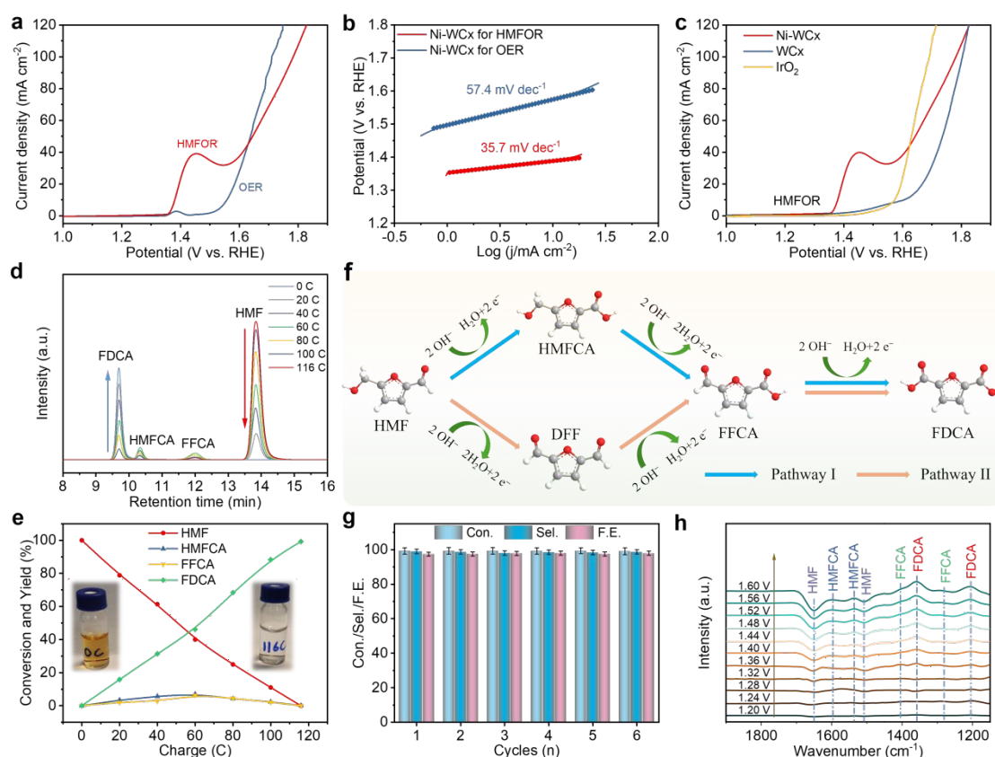
Figure 3. Electrocatalytic HMFOR performance evaluations. (a) LSV curves of Ni-WC x in 1 M KOH with and without 20 mM HMF, and (b) corresponding Tafel plots. (c) LSV curves illustrating the HMFOR performance of Ni-WC x , WC x and IrO 2 . (d) HPLC curves with increasing charge accumulation at 1.45 V vs. RHE. (e) Charge-dependent concentration for HMF, FDCA, HMFCA, and FFCA. (f) Two principal reaction pathways for oxidation of HMF to FDCA. (g) Conversion, selectivity and Faradaic efficiency for FDCA production over six sequential electrolysis cycles. (h) In situ FTIR spectra of Ni-WC x obtained at various applied potentials during HMFOR.
