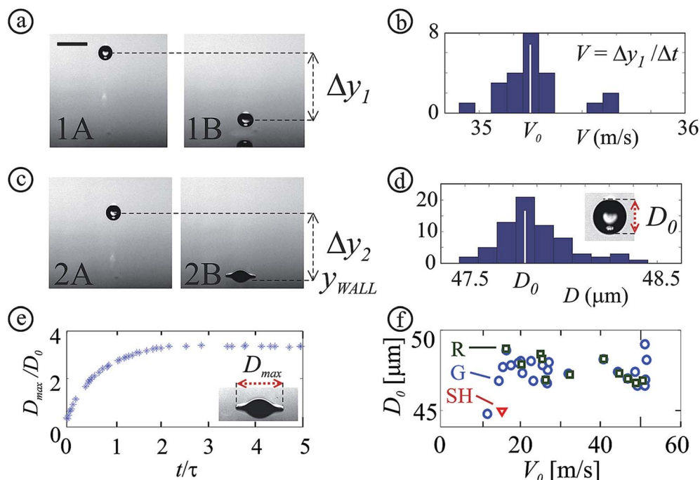
Fig. 4 Determination of droplet size and velocity. All images shown are for equal droplet generation settings. (a) Two in-flight frames are used to determine the droplet translation \Delta y_1 . The translation is used to obtain the droplet velocity. The scale bar indicates 100 \mu\text{m} . (b) Velocity histogram. The median provides the impact velocity V_0 . Here and in (d), note the scale of the velocity axis: the distribution is very narrow. (c) Droplet captured in-flight (frame 2A) and during spreading (frame 2B). Frame A is used to collect the diameter D for each experiment. (d) Diameter histogram. The median provides the droplet diameter for each experimental setting, D_0 . (e) Example curve of D_{\text{max}}/D_0 is plotted versus time. The maximum spreading diameter D_{\text{max}} is determined from frame 2B. (f) Parameter space of D_0 and V_0 . The markers indicate the surface type (G: glass ( \theta = 23^\circ ), R: RainX ( \theta = 90^\circ ), SH: superhydrophobic ( \theta = 135^\circ )).
