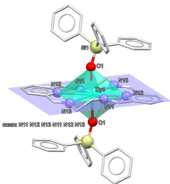
Fig. 2 Balls and sticks diagram for the cation [\text{Dy}(\text{L}^{\text{N}6\text{en}})(\text{OSiPh}_3)_2]^+ in the \{[\text{Dy}(\text{L}^{\text{N}6\text{en}})(\text{OSiPh}_3)_2](\text{BPh}_4)\} complex 1a , showing Dy1 as a polyhedron. Only heteroatoms of the asymmetric unit and those corresponding to the coordination sphere are labelled.
