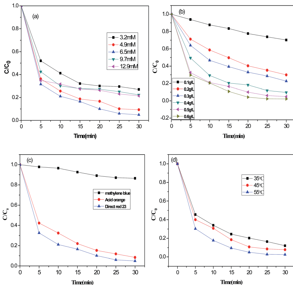
Fig. 6 Effects of experimental factors on DR23 degradation: (a) \text{H}_2\text{O}_2 concentration (reaction conditions: temperature, 25^\circ\text{C} ; catalyst loading, 0.5\text{ g L}^{-1} ; initial dye concentration, 0.02\text{ g L}^{-1} ), (b) catalyst loading ( \text{H}_2\text{O}_2 concentration, 6.5\text{ mM} ; initial dye concentration, 0.02\text{ g L}^{-1} ; and neutral pH), (c) type of dye (temperature, 25^\circ\text{C} ; catalyst loading, 0.5\text{ g L}^{-1} ; \text{H}_2\text{O}_2 concentration, 6.5\text{ mM} ; initial dye concentration, 0.02\text{ g L}^{-1} ), and (d) temperature (catalyst loading, 0.5\text{ g L}^{-1} ; \text{H}_2\text{O}_2 concentration, 6.5\text{ mM} ; initial dye concentration, 0.06\text{ g L}^{-1} ).
