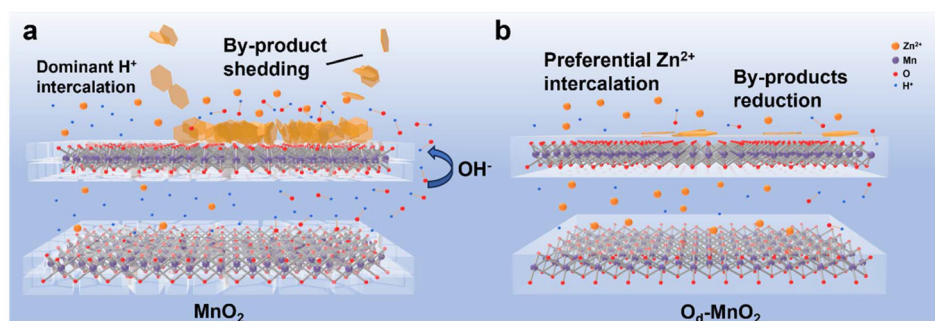
Fig. 1 The schematic diagram of the ion intercalation process of (a) \text{MnO}_2 and (b) \text{O}_\delta\text{-MnO}_2 .
