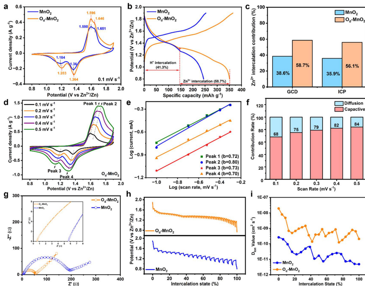
Fig. 3 Electrochemical kinetics of Zn/ \text{MnO}_2 and Zn/ \text{O}_\text{d}\text{-MnO}_2 batteries. (a) CV curves at 0.1 \text{mV s}^{-1} . (b) Galvanostatic charge/discharge curves at 0.1 \text{A g}^{-1} . (c) The percentage of \text{Zn}^{2+} intercalation contribution calculated by GCD and ICP. (d) CV curves at different scan rates, (e) Determination of the b value using the relationship between the peak current and scan rate, and (f) the corresponding percent of the pseudocapacitive contribution of the Zn/ \text{O}_\text{d}\text{-MnO}_2 battery. (g) EIS spectra, with a larger view of the equivalent series resistance in the inset. (h) GITT curves and (i) the corresponding ion diffusion coefficients.
