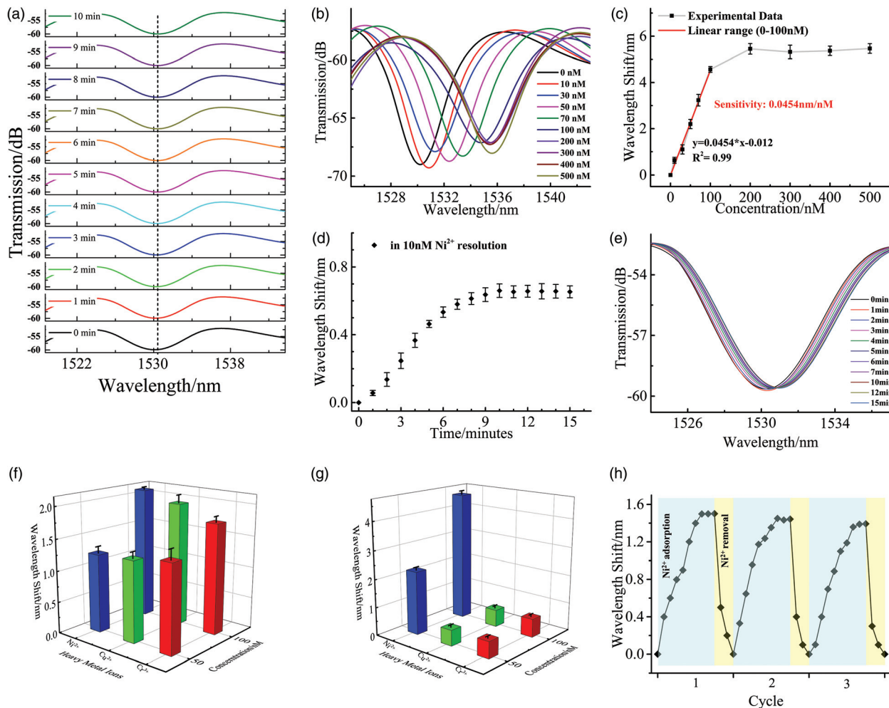
Fig. 3 (a) Spectral response curves of the STNCS sensor coated with Ni 2+ -II-CS and immersed in DI water for 10 min (the standard deviation is 0.098 nm). (b) Spectral response curves of the STNCS sensor coated with Ni 2+ -II-CS to different Ni 2+ ion concentrations. (c) Ni 2+ ion calibration curve and linear response of the STNCS sensor coated with Ni 2+ -II-CS film. (d) Response time curves of the STNCS sensor coated with Ni 2+ -II-CS and immersed in 10 nM Ni 2+ solution. (e) Spectral response of the STNCS sensor coated with Ni 2+ -II-CS to 10 nM Ni 2+ ion solution for 15 min. (f) Response of the STNCS sensor coated with Ni 2+ -NII-CS to different concentrations (50 and 100 nM) of heavy metal ions (nickel, copper, and chromium). (g) Response of the STNCS sensor coated with Ni 2+ -II-CS to different concentrations (50 and 100 nM) of heavy metal ions (nickel, copper, and chromium). (Error bars represent standard deviations for three parallel experiments). (h) Regeneration cycle: shift in dip wavelength of the STNCS sensor coated with Ni 2+ -II-CS caused by sequential exposure to 50 nM Ni 2+ solution and MES buffer.
