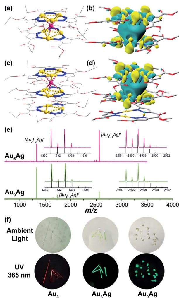
Fig. 1 Crystal structures for (a) \text{Au}_6\text{Ag} and (c) \text{Au}_9\text{Ag} and molecular orbital contours of the LUMOs for (b) [\text{Au}_6\text{Ag}]^+ and (d) [\text{Au}_9\text{Ag}]^+ (vide infra, isovalue = 0.02). Hydrogens, counteranions \text{PF}_6^- , and disordered sets in the \text{Au}_3 rings and Ag cations are omitted from the figures for clarity. (e) MALDI-TOF-MS spectra of (top) \text{Au}_6\text{Ag} and (bottom) \text{Au}_9\text{Ag} . Inset: simulated and measured isotopic distributions of (left) [\text{Au}_3\text{L}_3\text{Ag}]^+ and (right) [\text{Au}_6\text{L}_6\text{Ag}]^+ fragments. (f) Digital photographs of crystals of \text{Au}_3 , \text{Au}_6\text{Ag} and \text{Au}_9\text{Ag} under ambient and 365 nm UV light, respectively.
