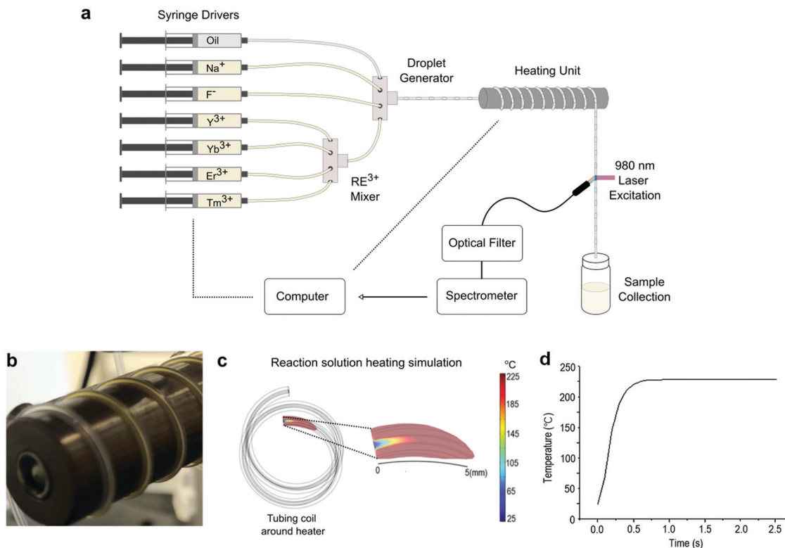
Fig. 1 (a) Schematic of the droplet-based microfluidic platform with inline infrared laser (980 nm) PL detection for NaYF 4 :Yb,Er,Tm UCNP synthesis. The microfluidic platform incorporates syringe pumps, a heating controller, and a real-time fluorescence detection system together. (b) Photograph of the heating loops around a 2 cm diameter heating rod. (c) Temperature distribution of the flow at the beginning of the heater, with temperatures of the heater and surrounding air at 220 °C and 25 °C, respectively. (d) Variation of the temperature of the reaction solution as a function of heating time.
