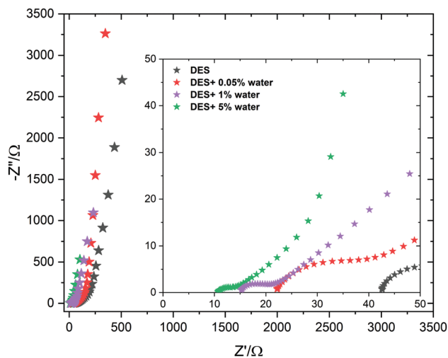
Fig. 8 Nyquist plots for the electrochemical capacitors operating in the DES and its water mixtures.
