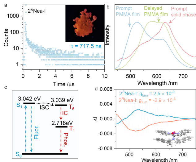
Fig. 6 (a) Emission decay curve of 2^R -Nea-I in the solid state, as well as the red emission under UV light (delay time = 50 \mu s). (b) Comparison of the emission spectra of 2^R -Nea-I in different states. (c) The Jablonski diagram. (d) CPL of 2^R -Nea-I measured in PMMA film. ( \lambda_{\text{ex}} = 350 nm).
