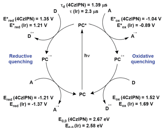
Fig. 8 Photocatalytic cycle comparing selected photophysical and redox properties of 4CzIPN and [\text{Ir}(\text{dF}(\text{CF}_3)\text{ppy})_2(\text{dtbbpy})]\text{PF}_6 in MeCN. 11,60,114,119–124
