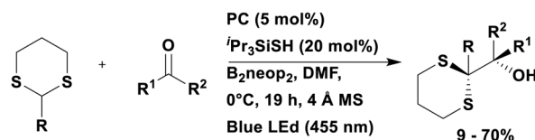
Fig. 208 Reaction scheme for the base-free Corey–Seebach reaction.
