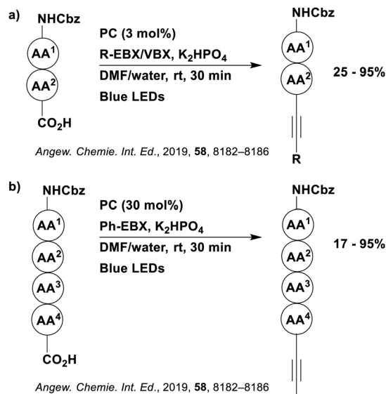
Fig. 142 Reaction scheme for the decarboxylative alkylation of (a) dipeptides and (b) peptide tetramers.
