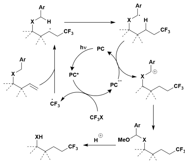
Fig. 42 Proposed mechanism for organic photoredox catalyzed synthesis of \delta -trifluoromethylated alcohols and amines where \text{X} = \text{O} or \text{NAr} .
