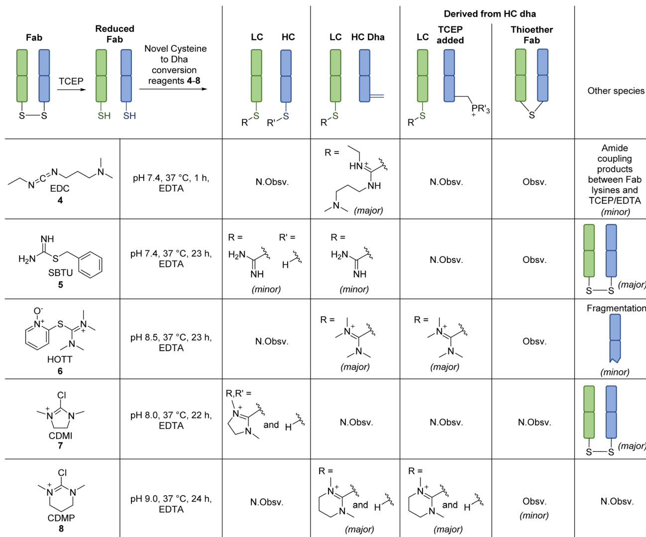
Scheme 2 Reaction of reagents capable of forming thiouronium with reduced Fab. Reactions were monitored by LC-MS. All reactions proceeded with complete conversion of the starting material Fab. N.Obsv. = Not Observed, Obsv. = Observed.
