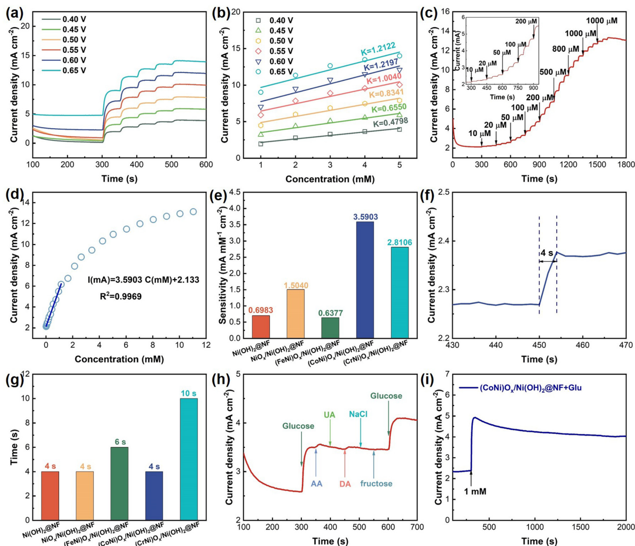
Fig. 5 (a) i – t curves of (CoNi) \text{O}_x /Ni(OH) _2 @NF at different voltages with incremental addition of 1 mM glucose. (b) The corresponding concentration–current fitting curves of (a). (c) i – t curve of (CoNi) \text{O}_x /Ni(OH) _2 @NF at a potential of 0.6 V (vs. Ag/AgCl) with addition of different concentrations of glucose. (d) The corresponding concentration–current fitting curve of (c). (e) The sensitivity of the prepared samples. (f) i – t curve of (CoNi) \text{O}_x /Ni(OH) _2 @NF with the addition of 10 \mu\text{M} glucose. (g) The current response time of the prepared samples. (h) i – t curve of (CoNi) \text{O}_x /Ni(OH) _2 @NF with the addition of glucose, AA, UA, DA, NaCl, and fructose. (i) Long-term stability of (CoNi) \text{O}_x /Ni(OH) _2 @NF with the addition of 1 mM glucose.
