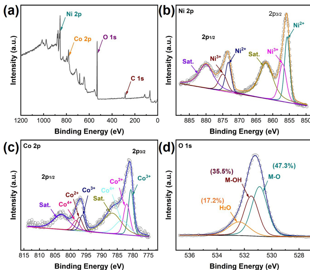
Fig. 3 (a) Survey spectra of (CoNi)O x /Ni(OH) 2 @NF. High-resolution XPS spectra: (b) Ni 2p, (c) Co 2p, and (d) O 1s.
