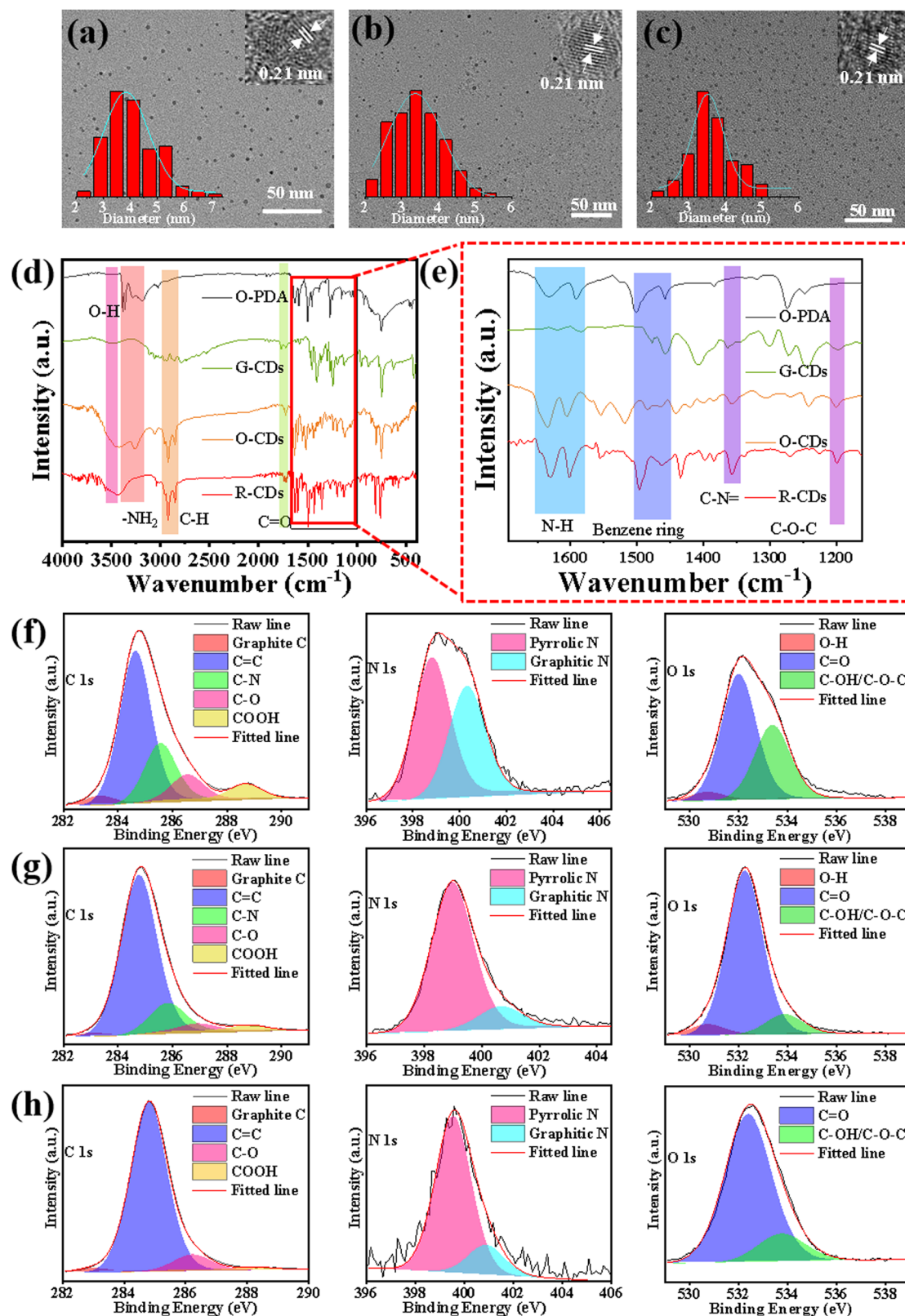
Fig. 2 Transmission electron microscopy (TEM) and corresponding diameter distribution histogram of (a) G-CDs, (b) O-CDs, and (c) R-CDs. (d) FTIR spectra and of O-PDA (black curve), G-CDs (green curve), O-CDs (orange curve), and R-CDs (red curve); (e) enlarged view of (d). High-resolution XPS C 1s, N 1s, and O 1s spectra of (f) G-CDs, (g) O-CDs, and (h) R-CDs.
