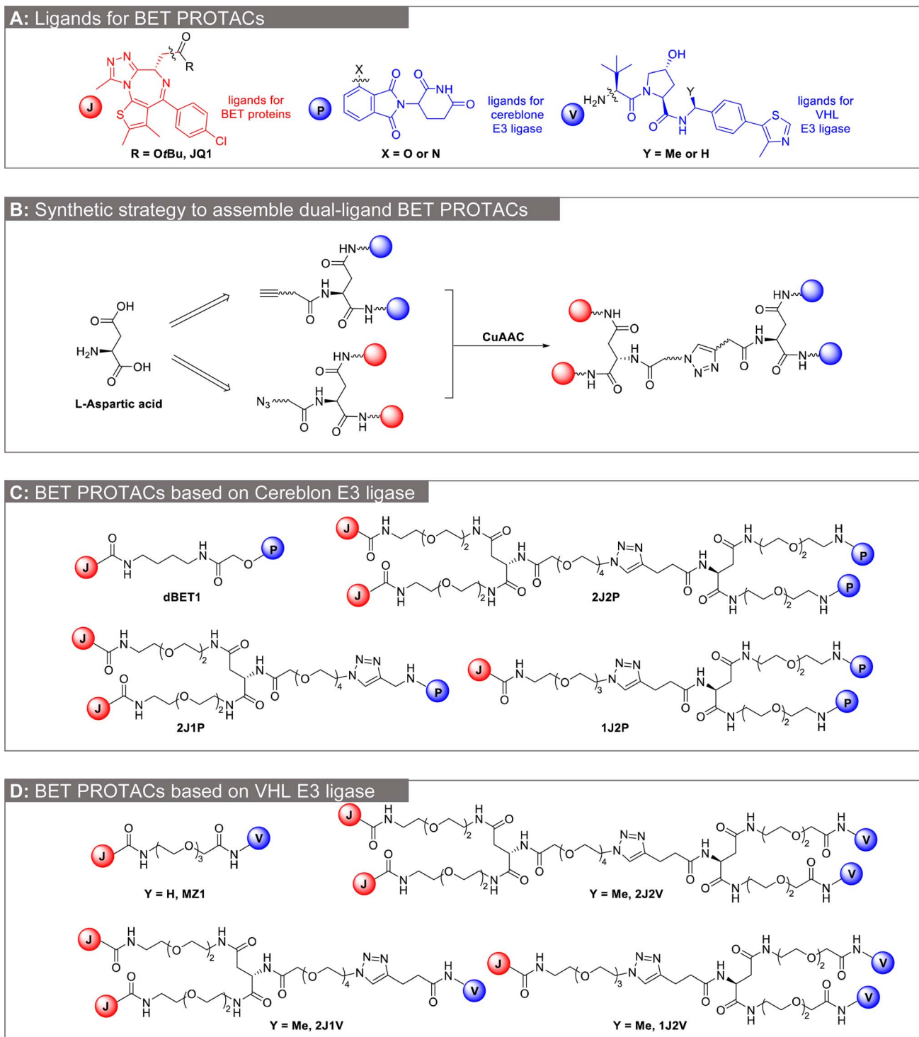
Fig. 2 Convergent synthesis of dual ligand BET PROTACs. (A) Chemical structure of the ligands used for the design of BET PROTACs. (B) General synthetic strategy to assemble the dual-ligand BET PROTACs. (C) Chemical structure of BET PROTACs based on pomalidomide for recruitment of the CRBN E3 ligase: dBET1 (single-ligand PROTACs), trivalent PROTACs (2J1P, 1J2P) and dual-ligand PROTACs (2J2P) (D) chemical structure of BET PROTACs based on VHL-ligand for recruitment of the VHL E3 ligase: MZ1 (single-ligand PROTACs), trivalent PROTACs (2J1V, 1J2V) and dual-ligand PROTACs (2J2V).
