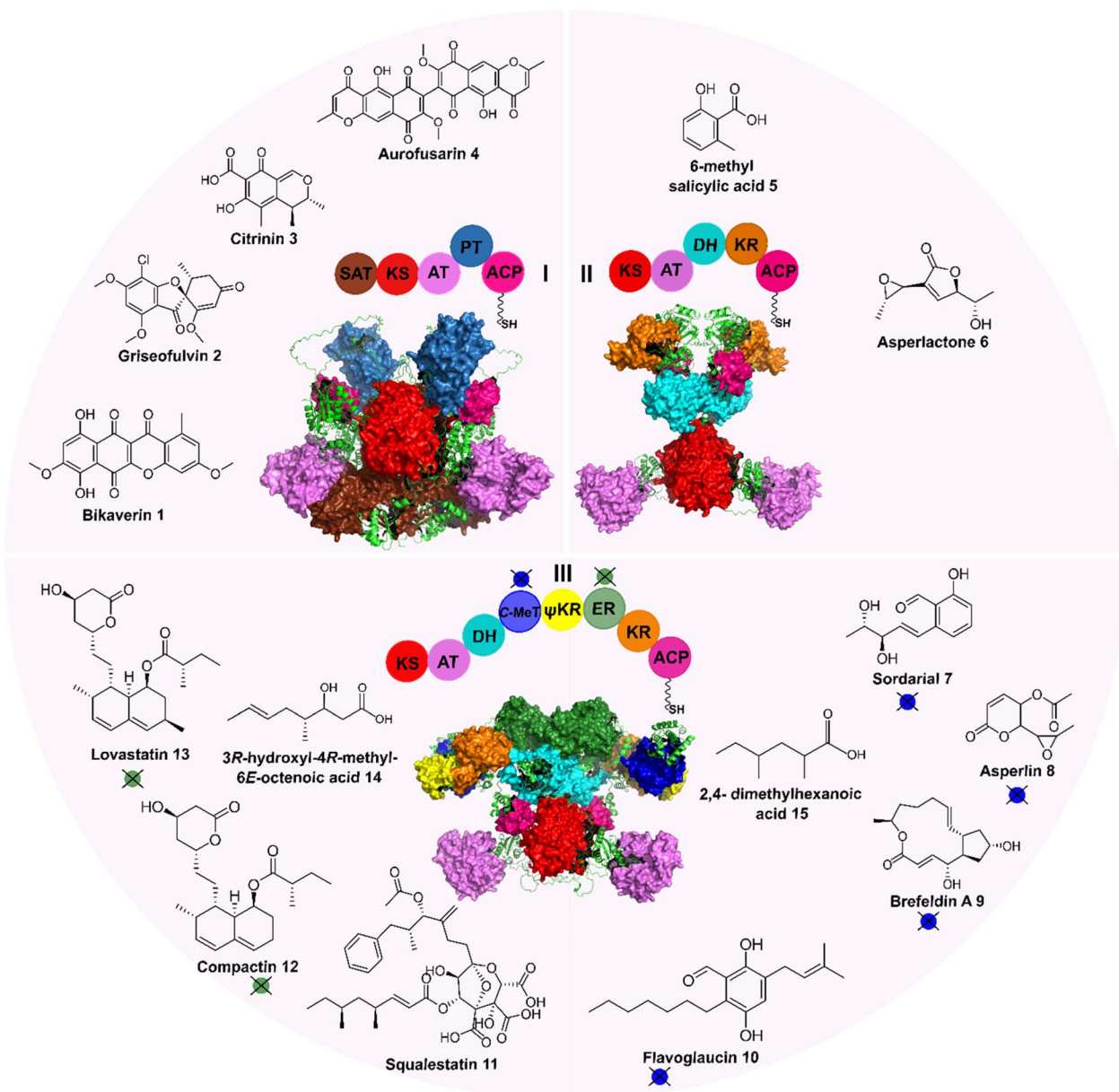
Fig. 2 Major types of fungal iPKSs and product examples. (I) SAT domain containing PKs, (II) partially reducing PKs, (III) highly reducing PKs. Compounds 11, 14, and 15 are the products of PKs with fully functional domains. Compounds 12 and 13 are produced by PKs with an inactive cis -ER domain, whereas compounds 7–10 are from PKs with a nonfunctional C-MeT domain. The blue and green circles with cross indicate inactive C-MeT and cis -ER domains respectively. PKs structures were generated using AlphaFold 3. 44
