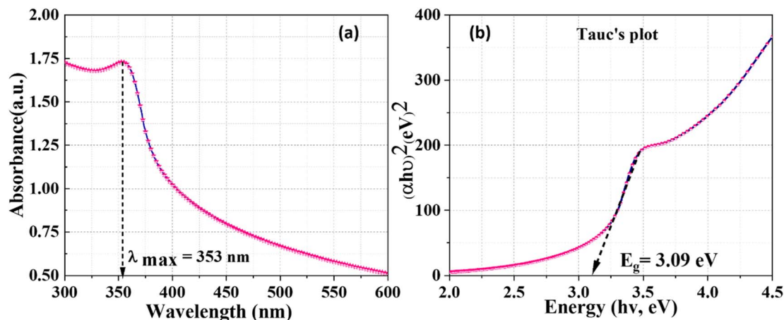
Fig. 3 Optical study J. adhatoda /ZnO NPs: (a) UV-visible absorption spectrum and (b) and Tauc plot.
