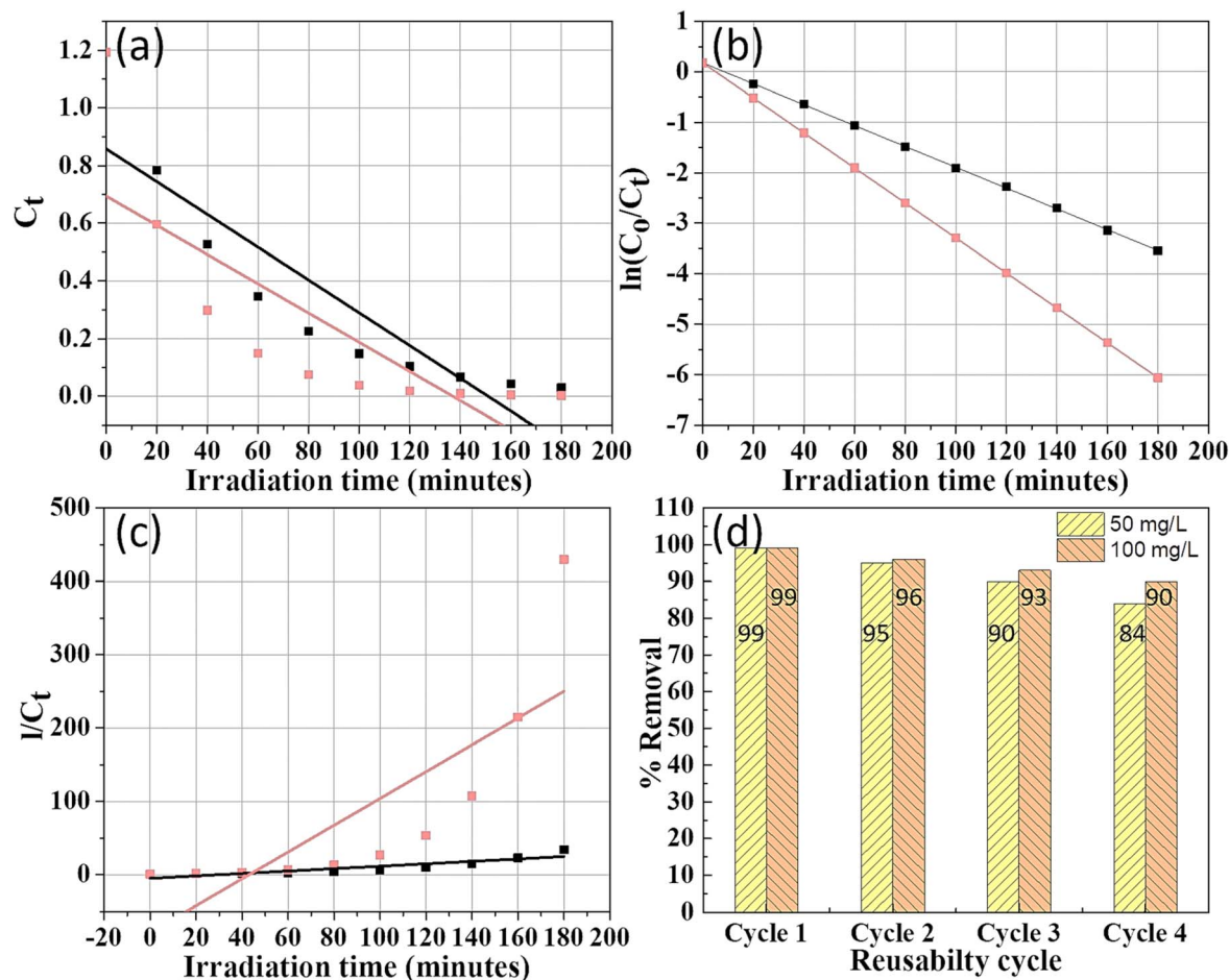
Fig. 13 Kinetics study of degradation of MG dye: (a) pseudo-zero-order, (b) pseudo-first-order, (c) pseudo-second-order, and (d) reusability J. adhatoda /ZnO NPs for the MG dye.
