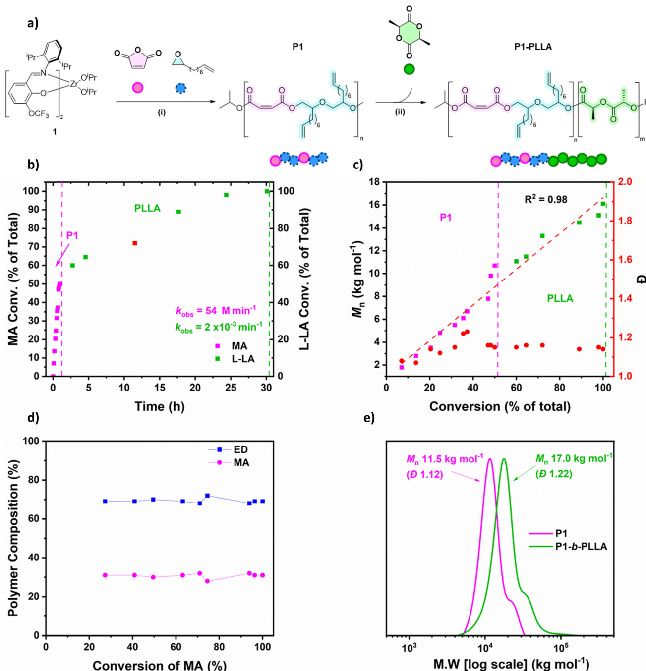
Fig. 1 Synthesis of poly(ester- alt -ether)- b -PLLA block polymers using catalyst 1 . (a) (i) The copolymerization of MA/ED, conditions: [MA]_0 = 0.5 \text{ mM} (50 equivalents), 50^\circ \text{C} in 1 mL epoxide (546 equivalents for ED), [1] = 0.01 \text{ mM} (one equivalent); (ii) L-LA polymerization, conditions: as before. The overall monomer stoichiometry is [1] : [MA] : [ED] : [L-LA] = 1 : 50 : 546 : 50 . (b) Conversion vs. time data for P1-PLLA formation, demonstrating MA (pink squares) and L-LA (green squares) conversion (normalised by overall maximum monomer conversion). The pseudo rate coefficients, k_{obs} , were determined as the gradient of the [MA] vs. time (min) for MA/ED ROCOP and the gradient of a plot of \ln([L-LA]/[L-LA]_0) vs. time (min) for L-LA ROP. (c) Plot showing P1-PLLA M_n and \bar{D} vs. monomer conversion. Data for the MA/ED ROCOP (pink), and then L-LA ROP (green). (d) Plot showing P1 composition vs. polymer conversion, with MA (pink) and ED (blue) conversions determined by ^1\text{H} NMR spectroscopy (Table 1). (e) GPC data for aliquots collected during P1-PLLA synthesis. The data show P1 formation (>99% conversion, pink) and, later, P1-PLLA formation (>99% L-LA conversion, green).
