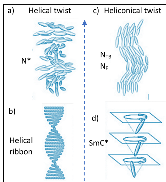
Fig. 2 Helical and helicoidal twist in LC phases: (a) and (b) helical is the uniform twist of the molecular long axis around a helix axis (dashed arrow) while (c) and (d) helicoidal twist takes place by precession of the tilt direction on a cone around the helix axis, occurring either in (a) and (c) nematic phases, or in (b) and (d) lamellar aggregates or smectic phases.
