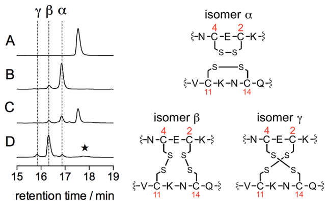
Fig. 3 HPLC monitoring of the reaction of \text{Zn} \cdot \text{L}_{\text{HSP}} (35 \mu\text{M} ) in a phosphate buffer (50 mM, pH 7.0, 298 K) with HOCl or \text{H}_2\text{O}_2 : chromatograms (A)–(D) correspond to unreacted \text{Zn} \cdot \text{L}_{\text{HSP}} (A), \text{Zn} \cdot \text{L}_{\text{HSP}} + 3.0 eq. HOCl (B), \text{Zn} \cdot \text{L}_{\text{HSP}} + 1.0 eq. HOCl (C) and \text{Zn} \cdot \text{L}_{\text{HSP}} + 3000 eq. \text{H}_2\text{O}_2 (D). The star on chromatogram (D) denotes \text{L}_{\text{HSP}} dimers with intermolecular disulfides. 28 The disulfide patterns of oxidation products \alpha , \beta and \gamma are shown on the right as identified by endopeptidase digestion and ESI-MS analyses.
