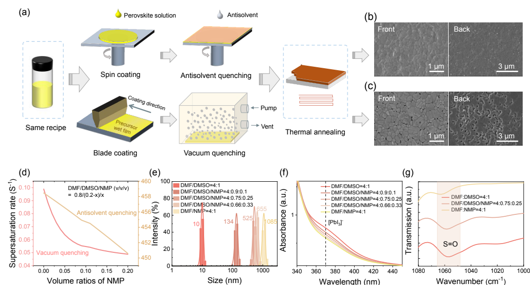
Fig. 1. (a) Schematic illustration of the vacuum quenching-assisted blade coating (VABC) and antisolvent-assisted spin coating (AASC) process. Top-view SEM images of the top surface and the back surface peeled from the perovskite/substrate bottom interfaces of films prepared by (b) AASC and (c) VABC. (d) Calculated supersaturation rate at the critical concentration for the DMF/DMSO/NMP solvent system with antisolvent quenching and vacuum quenching method. (e) Colloidal size distribution of the perovskite precursor solution in various DMF/DMSO systems after the addition of NMP, with the molar ratio relative to DMSO. (f) UV-vis absorption spectra of \text{PbI}_2 dissolved in DMF/DMSO with varying NMP volumes. (g) FTIR spectra of the intermediate powders obtained by vacuum-quenching, which were processed from DMF/DMSO, DMF/NMP, and DMF/DMSO/NMP.
