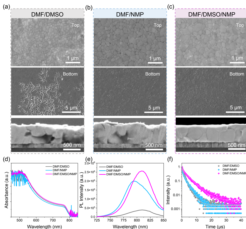
Fig. 3. SEM images of perovskite films processed from DMF/DMSO (a), DMF/NMP (b), and DMF/DMSO/NMP (c) solvent systems, (top panel: top surface, middle panel: buried interface; bottom panel: cross section). (d) UV-vis absorption, (e) Steady-state PL and (f) TRPL spectra of the perovskite films processed from the three solvent systems by VABC.
