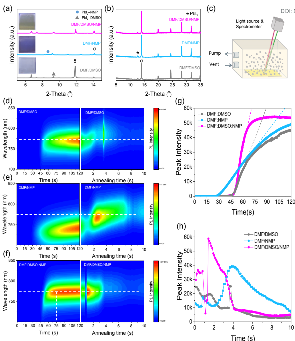
Fig. 2. (a) XRD patterns of the prepared intermediate films after vacuum quenching. (b) XRD spectra of the perovskite films after thermal annealing. (c) Schematic illustration of the vacuum quenching setup integrated with an in-situ optical monitor unit. Photoluminescence (PL) spectra evolution during the vacuum quenching stage (left) and thermal annealing process (right) for perovskite films blade-deposited from the three solvent systems: (d) DMF/DMSO, (e) DMF/NMP and (f) DMF/DMSO/NMP. Evolution of the PL peak intensity of the three films during (g) vacuuming and (h) annealing process.
