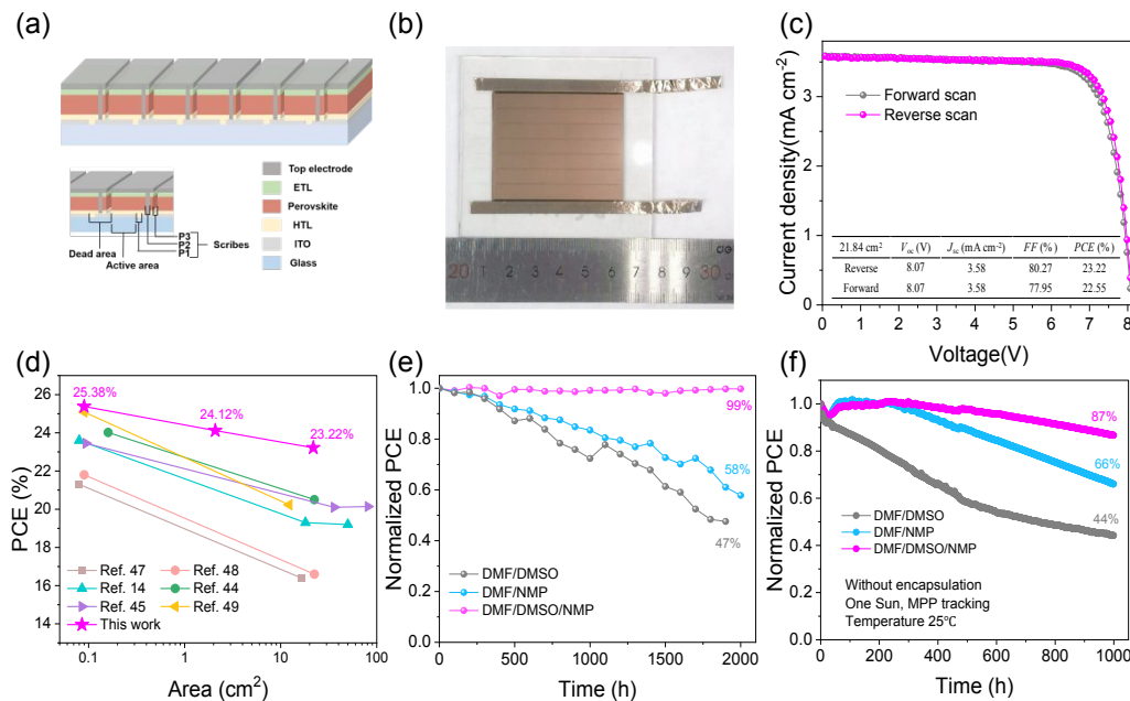
Fig. 5. (a) Schematic diagram of the perovskite mini-module. (b) Digital photograph and (c) J - V curves of the best-performing mini-module on 7.6 cm \times 7.6 cm substrate based on DMF/DMSO/NMP solvent system. (d) Comparison of efficiency decline during upscaling of the present work with those previously reported in literature 14, 44, 45, 47-49 . (e) Evolution of PCE of the unencapsulated blade-coated PSCs in an N_2 -filled glove box. (f) MPP tracking of PSCs under one sun illumination.
