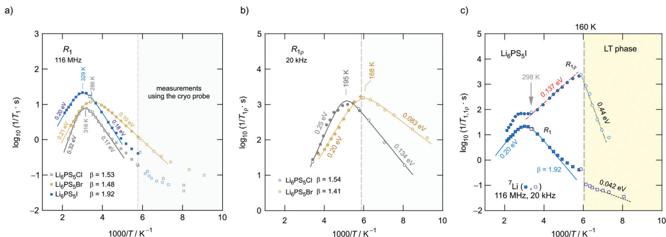
Fig. 11 (a) Temperature dependence of the diffusion-induced ^7\text{Li} NMR spin-lattice relaxation rates R_1 (116 MHz) of \text{Li}_6\text{PS}_5\text{X} (X = Cl, Br and I). Solid lines refer to BPP-type fits to extract activation energies and pre-factors. (b) Arrhenius plot of the corresponding ^7\text{Li} SLR \rho NMR rates recorded in the rotating frame of reference using a nominal locking frequency of \omega_1/2\pi = 20 kHz. Again, the solid lines represent fits according to a modified BPP relaxation model taking into account the asymmetry of the peaks by parameter \beta . The further the relaxation peak is shifted to lower T , the faster the Li exchange process inducing spin-lock spin-lattice relaxation. Therefore, Li diffusion, as seen by NMR, is increasing in the following order: \text{Li}_6\text{PS}_5\text{I} < \text{Li}_6\text{PS}_5\text{Br} < \text{Li}_6\text{PS}_5\text{Cl} (see also c). (c) R_1 and R_{1\rho} of \text{Li}_6\text{PS}_5\text{I} ; at 160 K \text{Li}_6\text{PS}_5\text{I} reversibly transforms into its low- T phase. At this temperature the rates R_1 show a jump toward lower values; the R_{1\rho} rates sharply decay with an activation energy of 0.44 eV. The unfilled symbols in (a–c) show rates measured with an NMR probe designed for experiments at cryogenic temperatures; the filled symbols refer to data which were acquired with a standard probe.
