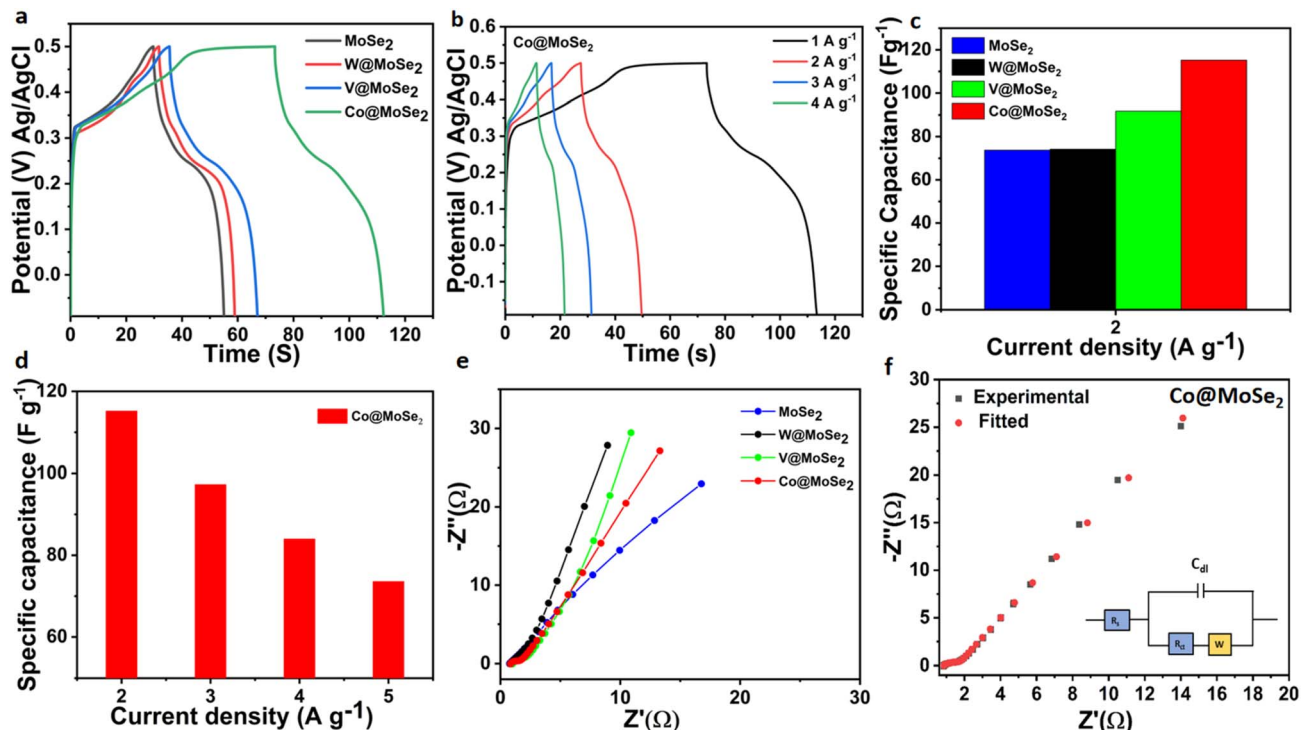
Fig. 6 (a) GCD plots for all samples at 1 A g -1 , (b) GCD plots of Co@MoSe 2 at varied current densities (A g -1 ), (c and d) current density vs. specific capacitance plots, (e) Nyquist plots corresponding to all prepared samples, and (f) experimental and fitted data for Co@MoSe 2 (the inset displays the equivalent fitted circuit).
