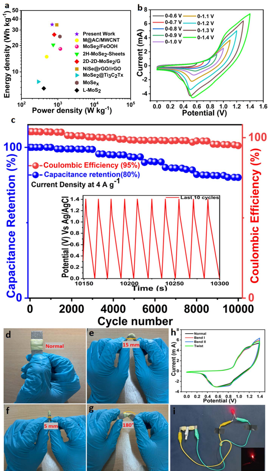
Fig. 8 (a) Ragone plot of the device compared with the reported literature, (b) CV curves observed over different potential windows, (c) cycling stability and coulombic efficiency of the \text{Co@MoSe}_2 SSD at a current density of 4 \text{ A g}^{-1} (the inset shows the GCD curves from the last ten cycles), (d–g) pictorial illustrations of the bending and twisting of the SSD and (h) related CV curves, and (i) photographic evidence of a red LED being lit by SSDs in series.
