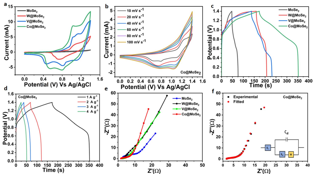
Fig. 7 Device mode: (a) comparative CV plots at a constant scan rate of 10 mV s -1 for all samples, (b) CV plots for Co@MoSe 2 at varied scan rates (10–100 mV s -1 ), (c) GCD plots for all samples at a current density of 1 A g -1 , (d) GCD plots of Co@MoSe 2 at current densities of 1, 2, 3, and 4 A g -1 , (e) Nyquist plots corresponding to all prepared samples, and (f) Nyquist plots for Co@MoSe 2 using both the experimental and fitted data (inset displays the equivalent fitted circuit).
