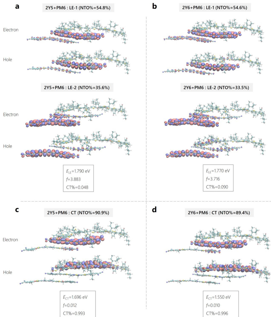
Fig. 7 Modelling of excited state energies for \text{H}_{\text{PM6}}:\text{Y}_x geometries. (a) and (b) Natural transition orbitals or NTOs (hole and electron) of the singlet local excited (LE) state in the 2Y5 + PM6 and 2Y6 + PM6 system. (c) and (d) NTOs of the charge transfer (CT) states for the same Y5- and Y6-based interfacial trimer systems. The two pairs NTOs of the LE state and one pair NTOs of the CT state are plotted, along with the corresponding weights (NTO%). The excitation energies ( E_{\text{LE}}/E_{\text{CT}} ), oscillator strength ( f ) and weight of CT character are provided as well.
