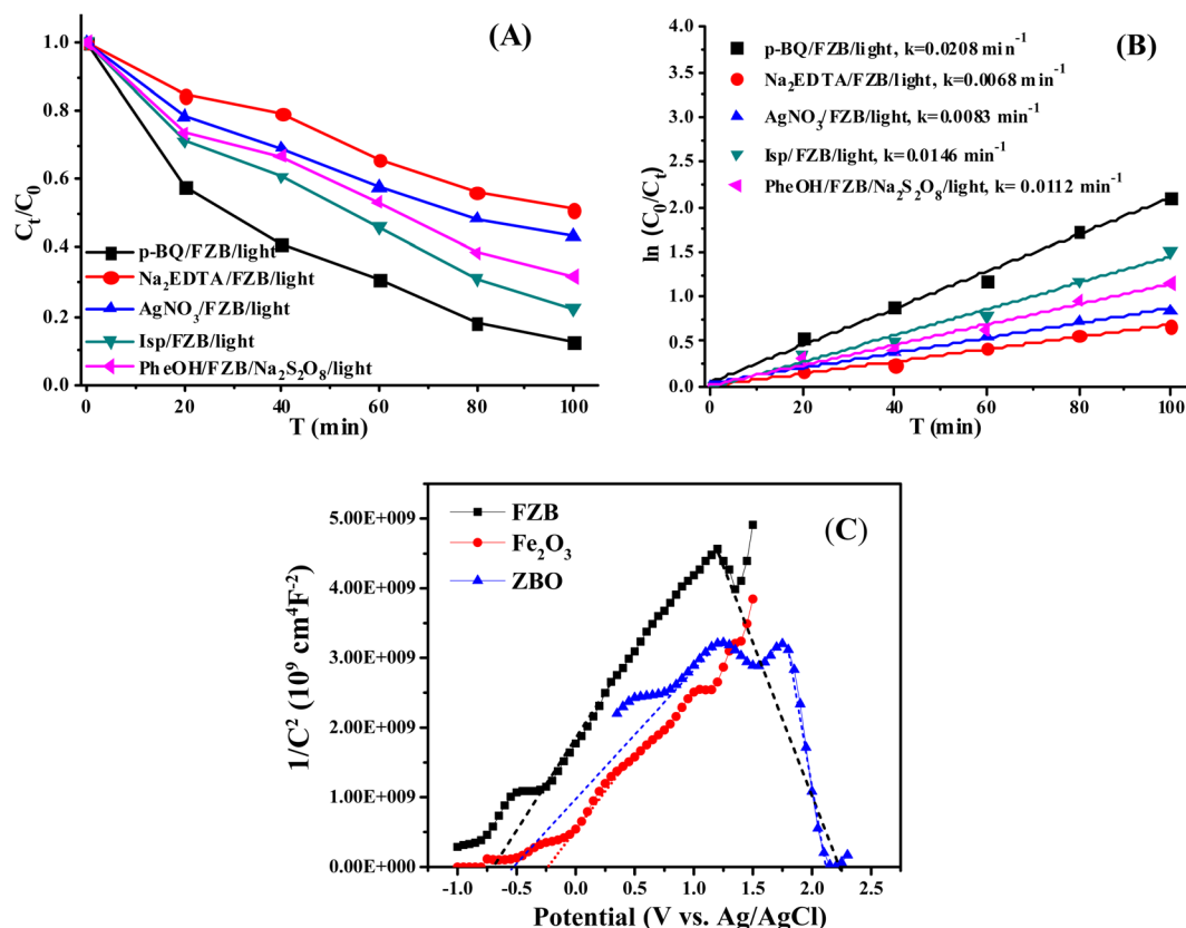
Fig. 8 Effect of radical scavengers (A and B) on MB degradation using FZB. (C) Mott–Schottky plots of \text{Fe}_2\text{O}_3 , \text{ZBO} , and \text{FZB} .
