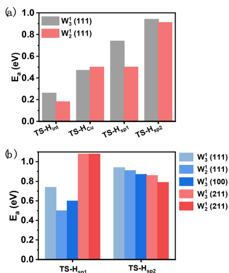
Fig. 6 (a) Comparison of the energy barriers of \text{H}_2 dissociation at the interface, Cu surface, and two hydrogen spillover processes on the \text{W}_3^1(111) and \text{W}_2^1(111) surfaces. (b) Comparison of energy barriers of the two hydrogen spillover processes at the interface of ZnO and different Cu crystal planes.
