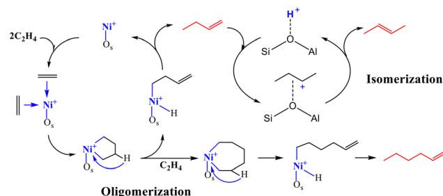
Scheme 11 Proposed catalytic cycles for linear ethylene oligomerization involving \text{Ni}^+ and \text{H}^+ as active sites on the Ni-AlSBA-15 catalyst ( \text{Os}_2^- = surface oxide ions). This scheme has been adapted from ref. 40.
