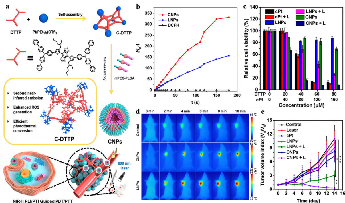
Fig. 20 (a) The designed C-DTTP metallacage. (b) ROS generation of LNP and CNP exposed to an 808 nm laser. (c) Cell viability of MDA-MB-231 cells after various treatments (L: 808 nm laser irradiation). (d) Thermal images of MDA-MB-231 tumor-bearing mice with different treatments. (e) Tumor volume growth curves of tumor-bearing mice with different treatments. Reproduced with permission from American Chemical Society, copyright 2022.99
