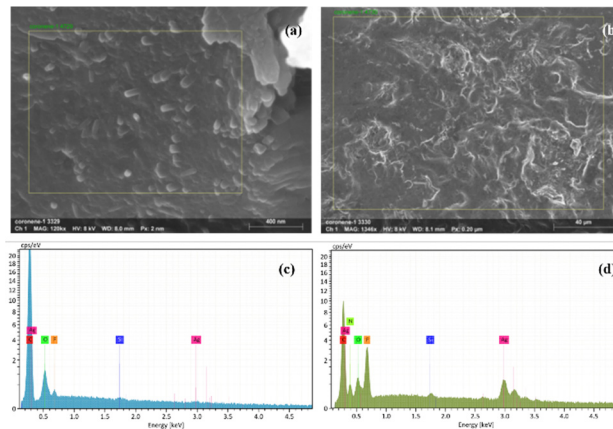
Fig. 5 SEM images of the adduct formed by \{[\mu-3,5-(\text{CF}_3)_2\text{pz}]\text{Ag}\}_3/\text{coronene} after dichloromethane LAG; (a) scan of spot 3; (b) scan of spot 4; (c) EDX analysis of spot 3; (d) EDX analysis of spot 4. Si, Al, and O are due to the mortar.
