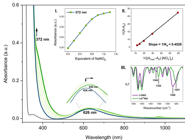
Fig. 2 UV-Vis spectral change upon addition of NaNO 2 . Grey line, 0.5 mM Terpy; teal blue line, 0.5 mM 1 . Stepwise addition of NaNO 2 is shown by the light green lines. Dark green line, spectrum after addition of 1 equiv. NaNO 2 . Inset I: rise of the band at 372 nm corresponding to NO 2 - coordination. Inset II: Benesi–Hildebrand plot for the binding constant calculation. Slope = 1/K_{\text{b}} = 0.4528 \text{ mM} . Inset III: FT-IR spectra of 1-ONO (violet line) and 1-O 15 NO (green line) in KBr.
