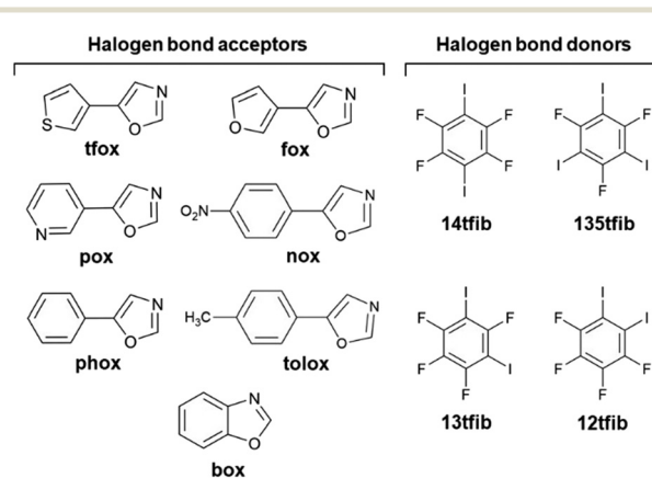
Scheme 1 Molecular structures of halogen bond acceptors and donors used in this study.
