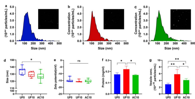
Fig. 2 Characterization of TELNs before and after tea fermentation. (a–c) Representative size distribution profiles and Brownian motion state of TELNs in the UF0 group (a), UF10 group (b) and AC10 group (c). (d–g) Comparison of (d) average size, (e) Zeta potential, (f) protein yield and (g) Vesicle concentration. "UF0", "UF10", and "AC10" represent the TELNs isolated from tea leaves at 0 days (unfermented), 10 days (unfermented), and 10 days (AC-fermented), respectively. AC, Aspergillus cristatus . All values are expressed as mean \pm SD (* p < 0.05 , ** p < 0.01 , ns: not significant; n = 7 ).
