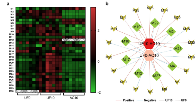
Fig. 4 Heatmap and correlation analysis (a) the relative contents of 30 differential metabolites in the UF0, UF10, and AC10 groups. The value of each compound was the result of Z-score transformation of its relative content. The metabolites not detected or had been below the detection limit in the corresponding sample were marked as "x" in the heatmap (b) correlation analysis between the contents of differential metabolites and the particles number of TELNs, |r| > 0.6 , p < 0.05 . Solid lines indicate significant correlations between metabolite relative abundance and particle number for the UF10 vs. AC10 group comparison; dashed lines indicate significant correlations for the UF0 vs. AC10 group comparison; red denotes a positive correlation and blue denotes a negative correlation. "UF0", "UF10", and "AC10" represent the TELNs isolated from tea leaves at 0 days (unfermented), 10 days (unfermented), and 10 days (AC-fermented), respectively. AC, Aspergillus cristatus .
