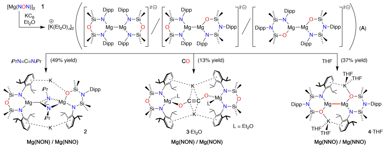
Scheme 2 Formation of A and reaction with i\text{PrN}=\text{C}=\text{NiPr} , \text{CO} and THF to afford 2 , 3 · \text{Et}_2\text{O} and 4 ·THF (isolated yields reported).
