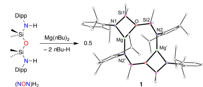
Scheme 1 Synthesis and thermal displacement plot (30% probability; H-atoms omitted; peripheral carbons as spheres) of 1 ( r = -x , 1 – y , – z ). Selected bond lengths (Å) and angles (°): Mg–N1 1.9414(10), Mg–O 2.0605(9), Mg–N2' 1.9542(10), Mg⋯Mg' 4.102(1); N1–Mg–O 77.54(4), N1–Mg–N2' 143.74(5), O–Mg–N2' 138.48(4).
