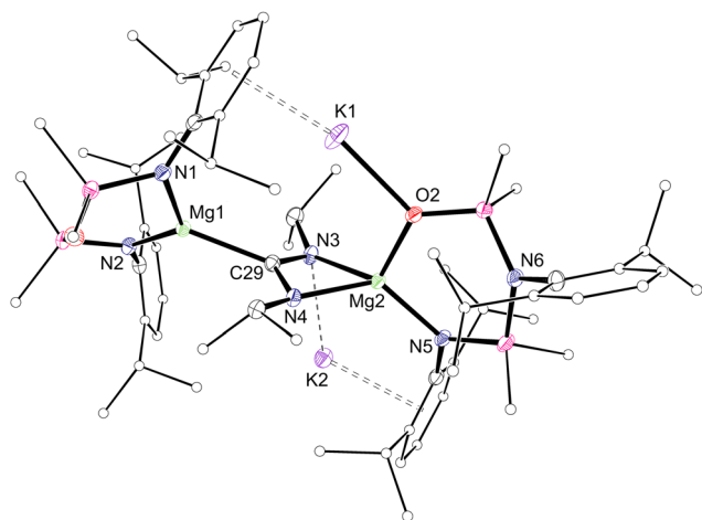
Fig. 2 Thermal displacement plot (30% probability; H-atoms omitted; peripheral carbons as spheres) of one of the independent molecules of 2 . Selected bond lengths (Å) and angles ( ^\circ ): \text{Mg1}-\text{N1} 2.0594(19), \text{Mg1}-\text{N2} 2.0415(19), \text{Mg2}-\text{N5} 2.0513(19), \text{Mg2}-\text{O2} 1.9122(16), \text{C29}-\text{N3} 1.358(3), \text{C29}-\text{N4} 1.344(3), \text{Mg1}-\text{C29} 2.232(2), \text{Mg2}-\text{N3} 2.1737(19), \text{Mg2}-\text{N4} 2.069(2); \text{N1}-\text{Mg1}-\text{N2} 123.18(8), \text{N5}-\text{Mg2}-\text{O2} 106.09(8), \text{N3}-\text{Mg2}-\text{N4} 63.51(7).
