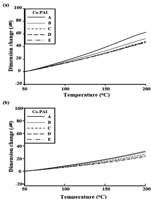
Fig. 3 TMA thermograms of Co-PAI films containing m -MPAB and (b) p -MPAB.
