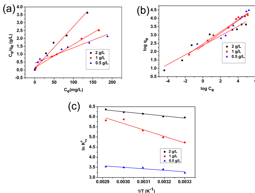
Fig. 7 (a) Langmuir and (b) Freundlich isotherms, and (c) plot of \ln K_{\text{eq}}^0 versus 1/T for fluoride ions adsorption.
