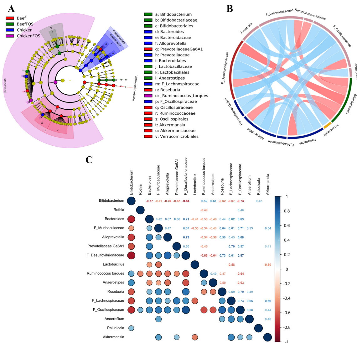
Fig. 3 Discriminant bacteria features across diets. (A) Cladogram representing the results of LfSe, highlighting taxa with significant differences among diets. (B) Network analysis of bacterial genera with strong correlations ( |r| \geq 0.65 ), showing positive (blue) and negative (red) correlations. (C) Spearman correlation matrix of discriminant bacteria at the genus level, displaying only statistically significant correlations. P -Values were corrected for multiple tests using the Benjamini–Hochberg procedure.
