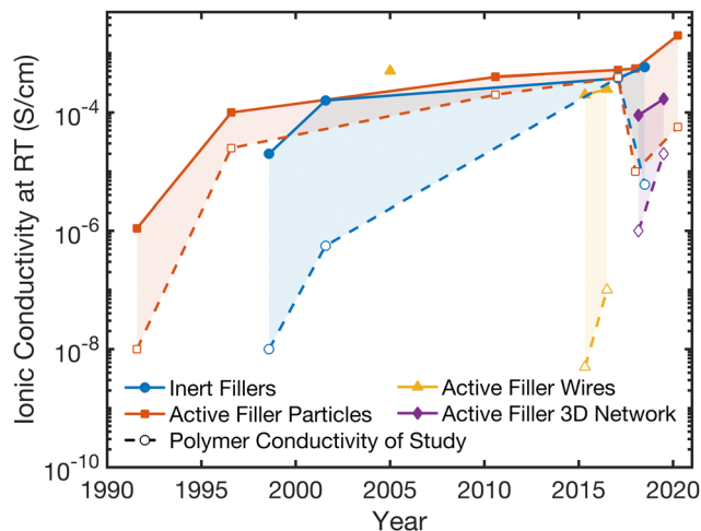
Fig. 3 Tracking of record composite electrolyte conductivities in each category and presenting the corresponding conductivity of the polymer electrolyte alone which was used in that study. The solid lines represent the record conductivity values over the years for each of the four composite categories, while the dashed lines show the polymer electrolyte conductivity alone that was shown in that study (if presented in the study). 27,28,48–50,64,69–77
