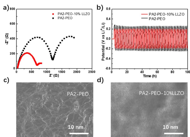
Fig. 4 EIS (a) of \text{LiFePO}_4 /PA2-PEO-10% LLZO/Li batteries, galvanostatic cycling of the symmetrical cell (b) 0.13 \text{ mA cm}^{-2} at 25 °C, and the SEM images (c and d) of Li metal anodes cycled with different SSEs.
