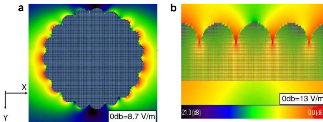
Fig. 43 (a) FDTD simulated electric-field distribution for a cauliflower-like Rh nanoparticle and (b) a flat Rh surface decorated with small nanohemispheres. The laser beam illuminates along the y-direction with x polarization. The scale bar is given at the bottom of (b). Figures are adapted from ref. 405 and 407 with permission. Copyright 2006 Springer Nature. Copyright 2006 Royal Society of Chemistry.
