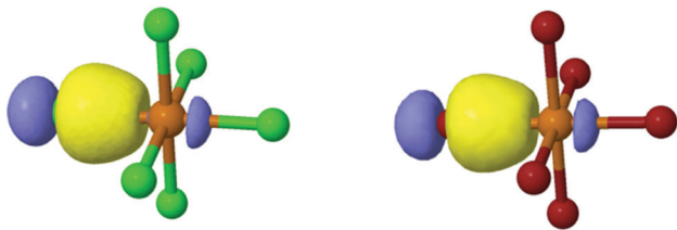
Fig. 12 Naturally localized atomic orbitals involved in Te–X bonding for (left) [TeCl_6]^{2-} and (right) [TeBr_6]^{2-} taken from 1 and 5 , respectively.
