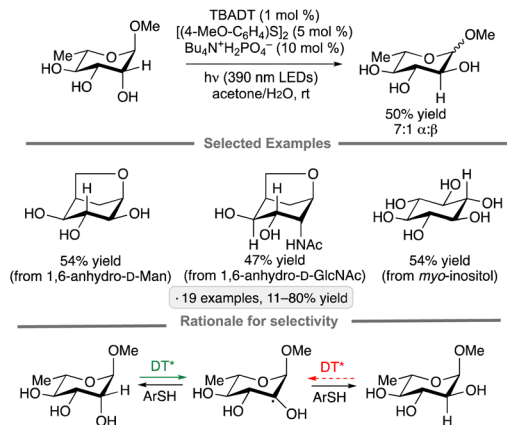
Scheme 60 Selective equatorial-to-axial epimerizations of OH groups. TBA denotes \text{Bu}_4\text{N}^+ ; DT denotes [\text{Bu}_4\text{N}^+][\text{W}_{10}\text{O}_{32}]^{4-} .
