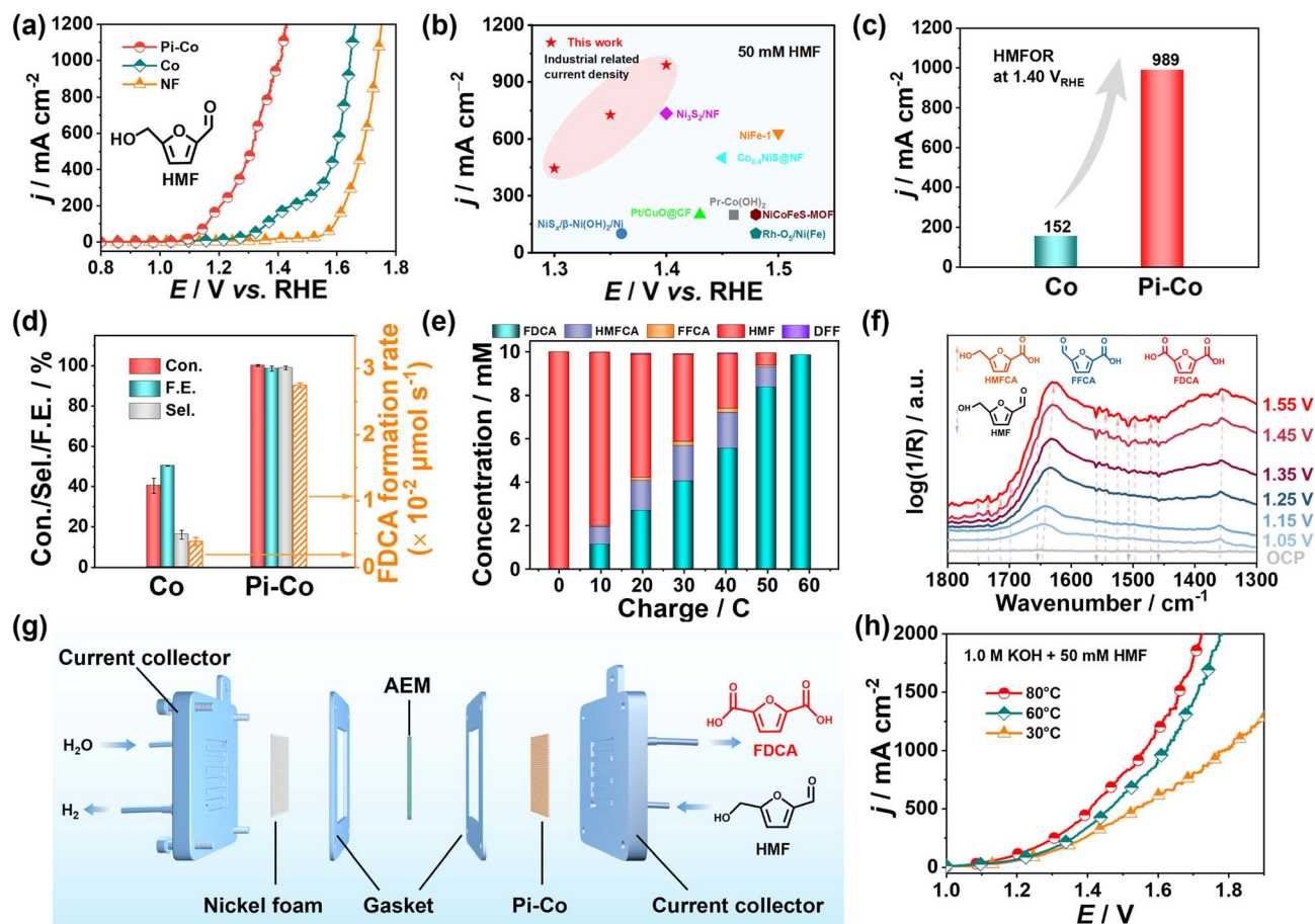
Fig. 3 (a) HMFOR LSV curves of Pi-Co and Co catalysts; (b) comparison performance with reported catalysts; (c) performance of Pi-Co and Co catalysts at 1.40 V_{RHE} ; (d) HMF conversion rates of Pi-Co and Co catalysts at 1.35 V_{RHE} for 3600 s; (e) concentration changes of reaction molecules at different charges; (f) in situ ATR-FTIR spectra of Pi-Co catalyst at different potentials; (g) schematic diagram of the AEM-based electrolyzer and (h) the corresponding LSV curves at different temperatures.
