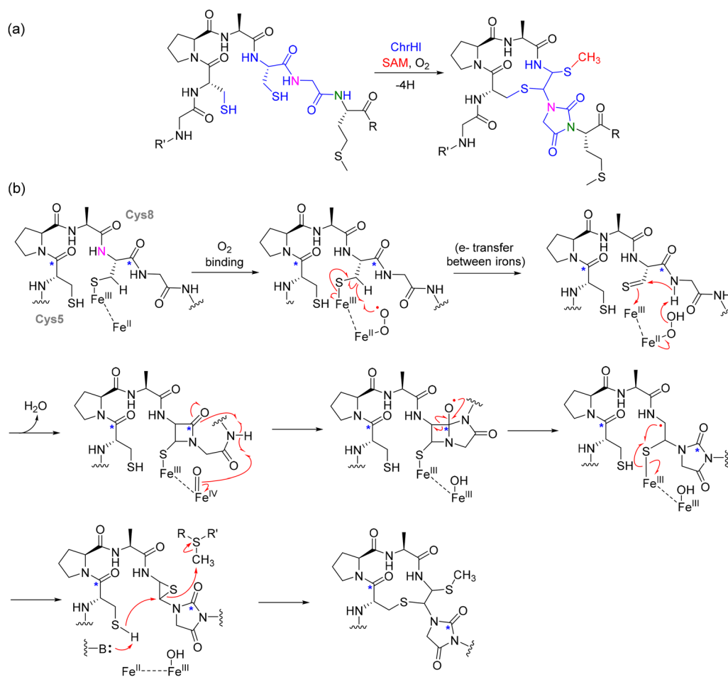
Fig. 31 Cyclization by the MNIO protein ChrH. (a) ChrH is a non-heme iron-dependent DUF692 enzyme that together with its membrane-bound partner ChrI transforms a linear peptide into a macrocycle, an imidazolidinedione, and a methylated thioaminal. (b) Proposed mechanisms of the cysteine modifying MNIO ChrH. Blue asterisks (*) indicate the carbon atoms that were isotopically labeled in the feeding experiments, corresponding to the carbonyl carbon of Cys8 and the β-carbon of Cys5. These labels were used to trace the fate of the carbon atoms in the product structure.
