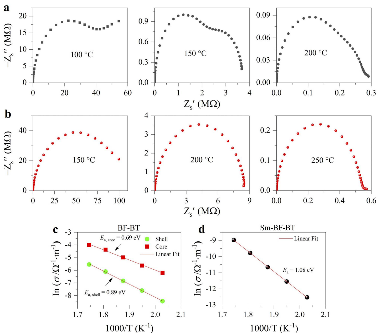
Fig. 6 The high-temperature impedance and defect chemistry analysis. Impedance complex plane plots for the undoped (a) and doped (b) samples at various temperatures. (c) Core and shell conductivities of the BF–BT ceramic. (d) Bulk conductivity of the Sm-doped BF–BT ceramic. The solid line is a result of linear least-square fitting.
