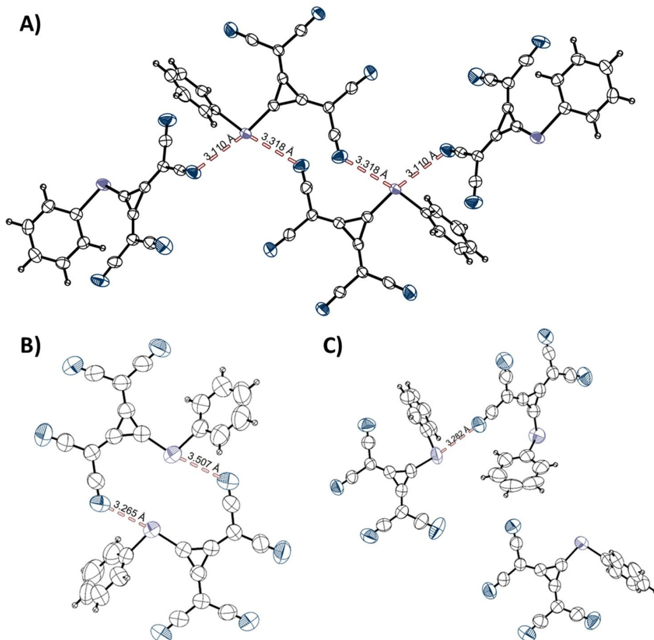
Figure 4: Single crystal X-ray structure of 8 : A - Biaxial binding; B , C - monoaxial binding. The sum of van-der-Waals radii for selenium and nitrogen amounts to 3.45 Å. TDA cations omitted for clarity. Ellipsoids set at 50% probability. In both cases of monoaxial binding, the formation of the chalcogen-bond is observed in the elongation of the cyclopropanide-selenium bond. In A , suitable interactions are detected along both axes. The bond formed in the elongation of the cyclopropanide substituent is significantly shorter. A summary of observed bond lengths and angles can be found in Table 1.
