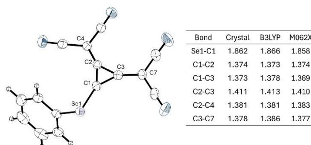
Figure 2. Selected average bond lengths of 8 . Ellipsoids set at 50% probability. TDA cations omitted for clarity. Geometry optimization performed with B3LYP 20 and M06-2X 21 functionals, applying def2TZVP(D) 22 basis set.
