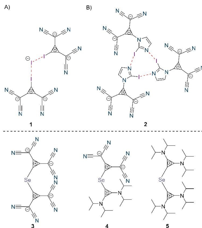
Figure 1. Top: Previously reported cases of “anti-electrostatic” halogen bonded aggregates of 1,2-bis(dicyanomethylene)-cyclopropanide-containing synthons in the solid state: A – 2:1 anion binding and B – trimer formation. For A : d_{I...I} = 85\% \Sigma r_w , in B : d_{I...N} = 79\text{--}81\% \Sigma r_w . Cations omitted for clarity. Bottom: Known cyclopropanide- and cyclopropenium-substituted chalcogen compounds. Counterions omitted for clarity.
