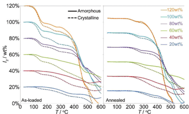
Fig. 11 The mass loss associated with I_2 release from the crystalline and amorphous ZIF-8 based by TGA of the as-loaded (left) and annealed (right) samples. This figure has been reproduced from ref. 87 with permission from the American Chemical Society, copyright 2011.
