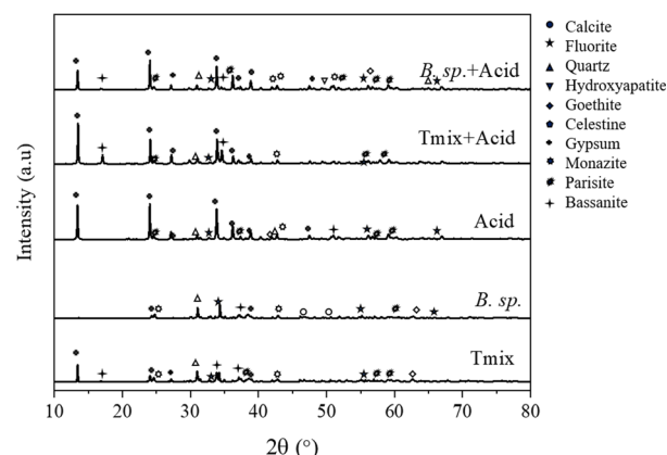
Fig. 6 XRD patterns after bio-pretreatment and acid leaching.
